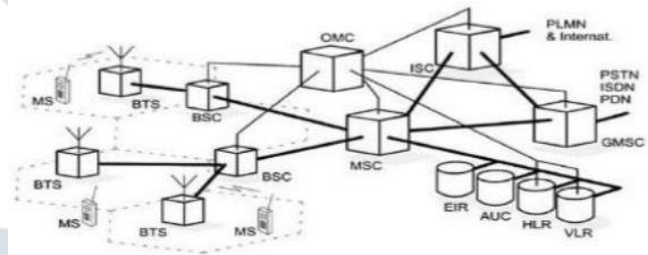
Figure 1. Architecture of GSM Technology
